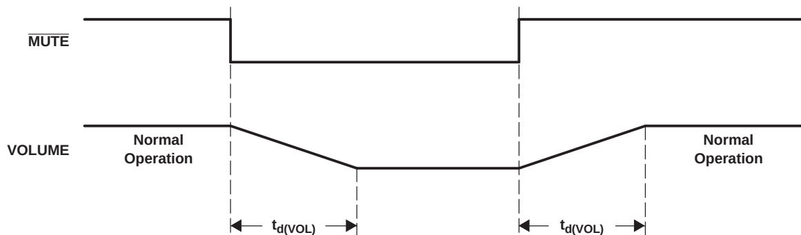
Figure 3-8. Mute Timing
