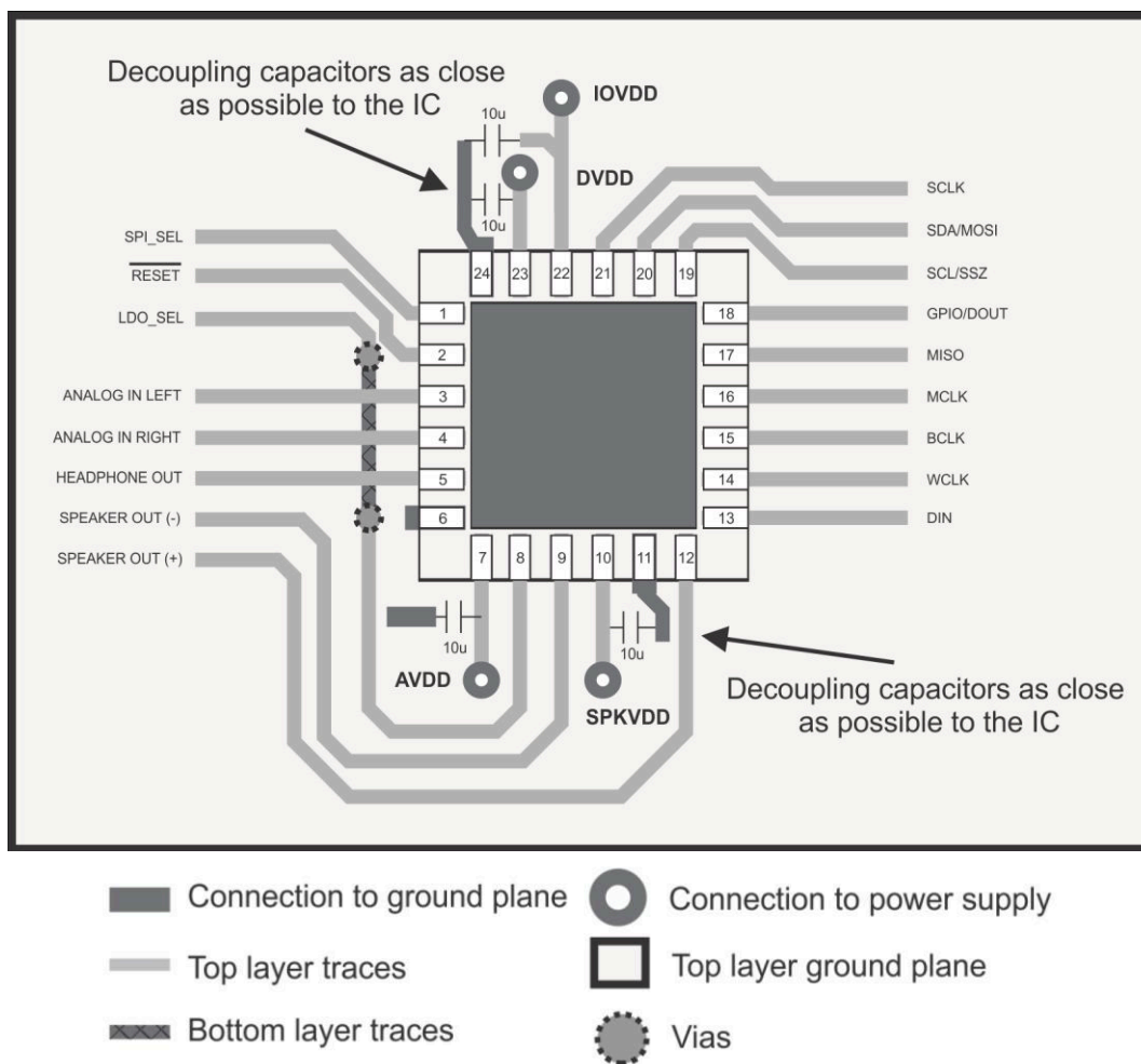
Figure 9-5. Layout Diagram
