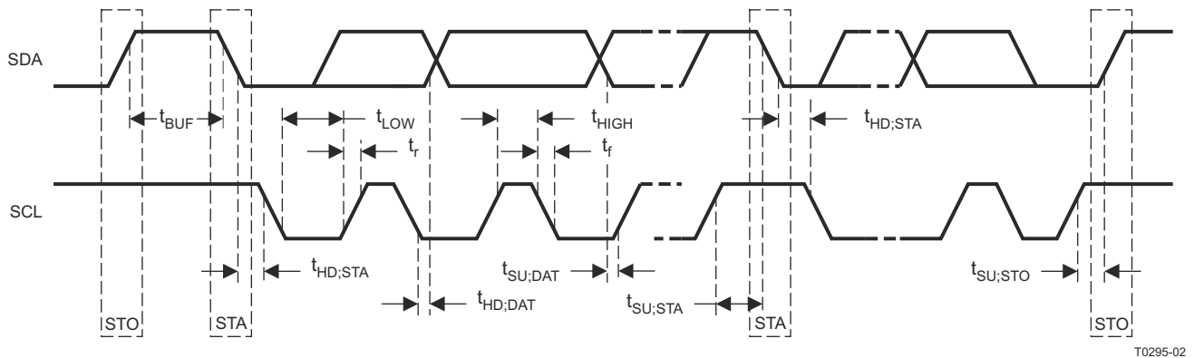
Figure 5-5. I²C Interface Timing
