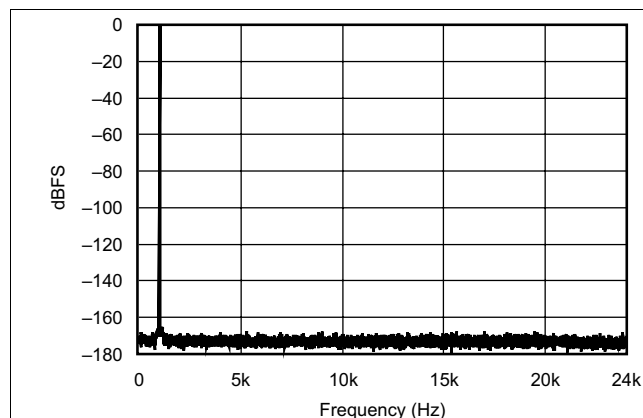
Figure 78. FFT With 1-kHz Input Tone at 0 dBFS
