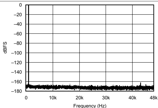
Figure 5. FFT With 1-kHz Input Tone at 0 dBFS
