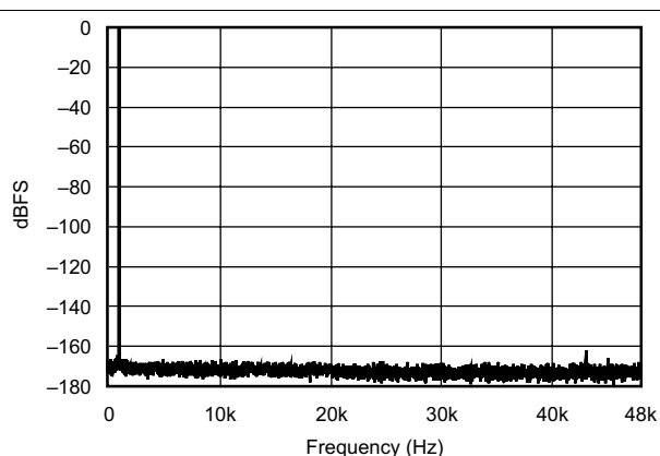
Figure 79. FFT With 1-kHz Input Tone at 0 dBFS
