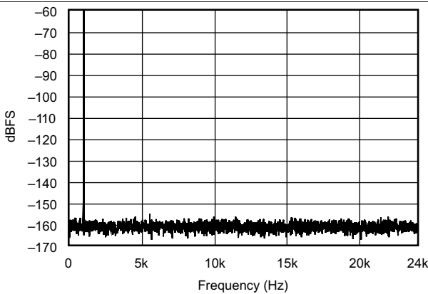
Figure 30. FFT With 1 kHz Input Tone at -60 dBFS (192 kHz:48 kHz)
