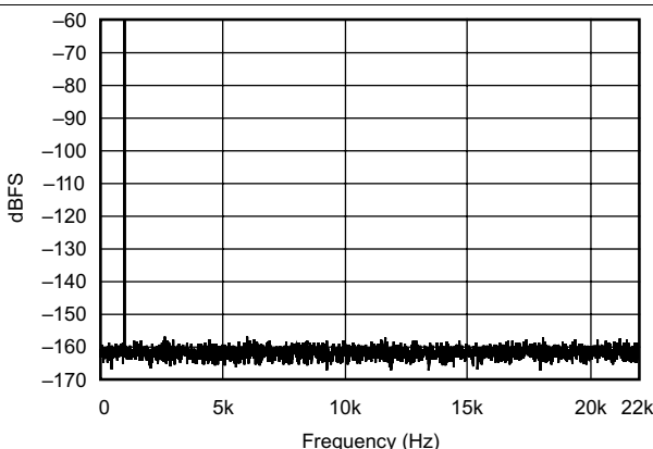
Figure 28. FFT With 1 kHz Input Tone at -60 dBFS (192 kHz:44.1 kHz)
