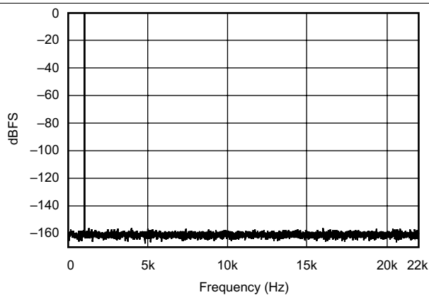
Figure 11. FFT With 1 kHz Input Tone at 0 dBFS (48 kHz:44.1 kHz)
