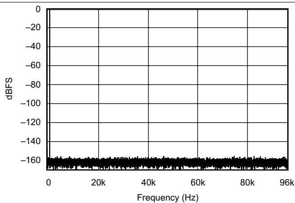
Figure 9. FFT With 1 kHz Input Tone at 0 dBFS (44.1 kHz:192 kHz)
