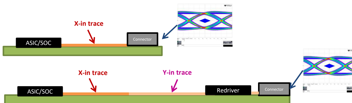
Figure 6-1. Linear Equalizer
