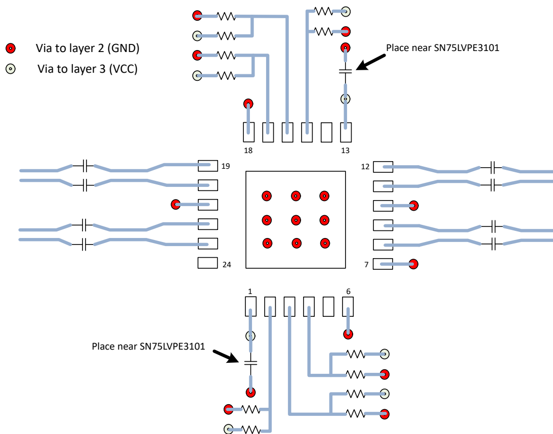
Figure 7-7. Example Layout
