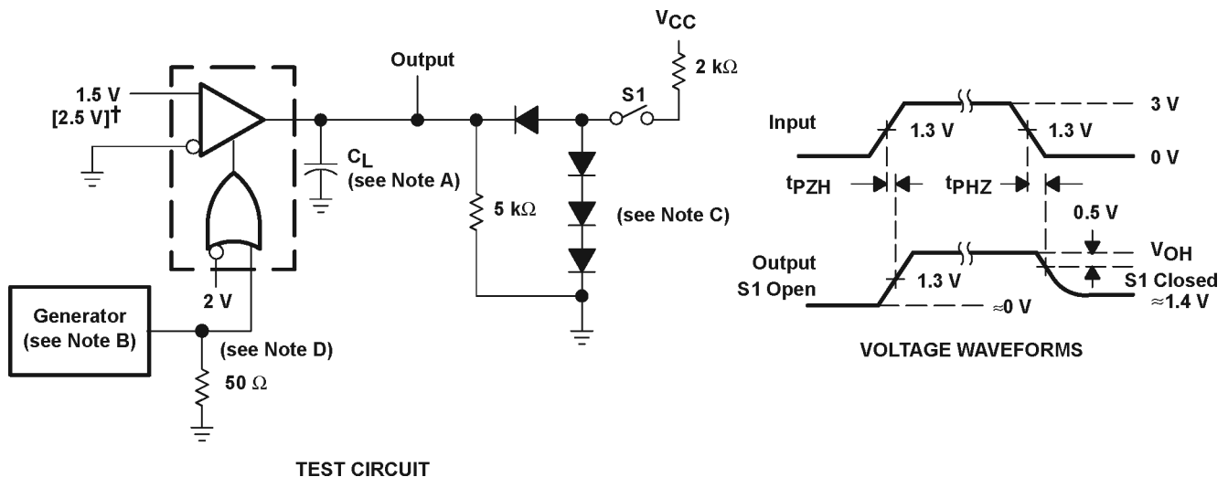
Figure 6-1. t_{PLH} , T_{PHL} Test Circuit and Voltage Waveforms
