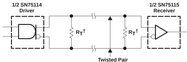
Figure 11. Basic Party-Line or Data-Bus Differential Data Transmission
