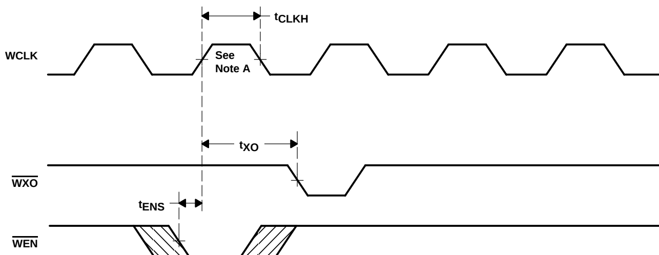
Figure 12. Write-Expansion-Out Timing
