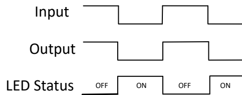
Figure 8-2. Application Curve
