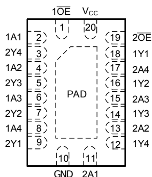
Figure 4-1. SN74LVC240A-Q1 RKS Package (Top View)
