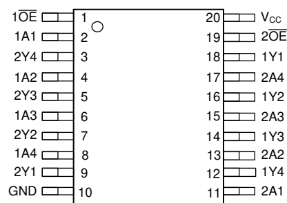
Figure 4-2. SN74LVC240A-Q1 PW, DGS Package (Top View)
