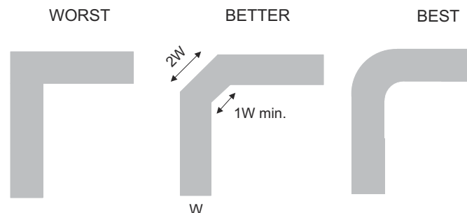
Figure 8-3. Trace Example
