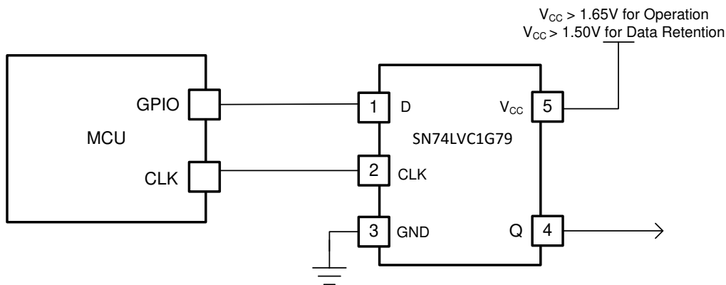
Figure 8-1. Low Voltage Data Retention With SN74LVC1G79
