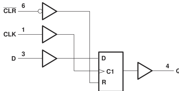
Logic Diagram
