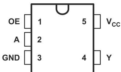
Figure 5-1. DCK or DBV Package, 5-Pin SC70 or SOT-23 (Top View)
