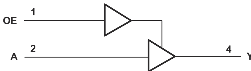
Figure 8-1. Logic Diagram
