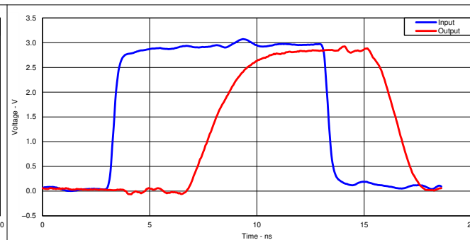
Figure 6-2. Switching Characteristics at 50 MHz Excellent Signal Integrity (3.3 V to 3.3 V at 3.3-V V_{CC} )
