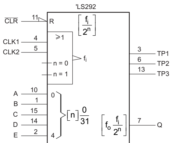
Figure 4. Logic Symbols
