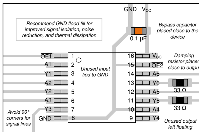
Figure 8-3. Example Layout for the SN74HCS365-Q1 in the PW Package
