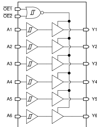
Figure 7-1. Logic Diagram (Positive Logic) for SN74HCS365-Q1
