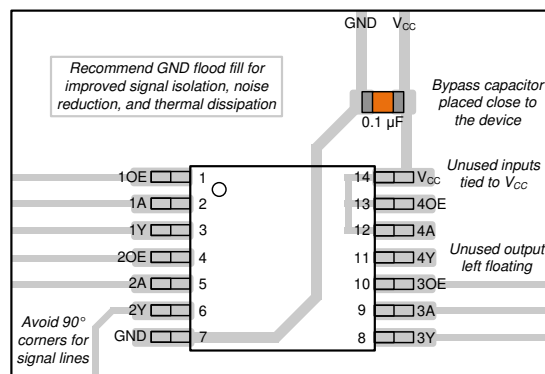
Figure 8-3. Example Layout for the SN74HCS126
