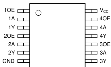
Figure 4-1. D, DYY, or PW; 14-Pin SOIC, SOT-23, or TSSOP Top View
