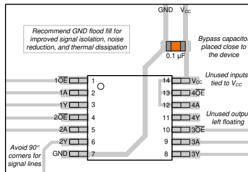
Figure 8-3. Example layout for the SN74HCS125-Q1
