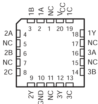
Figure 3-3. SN54ACT11 FK Package (Top View)
