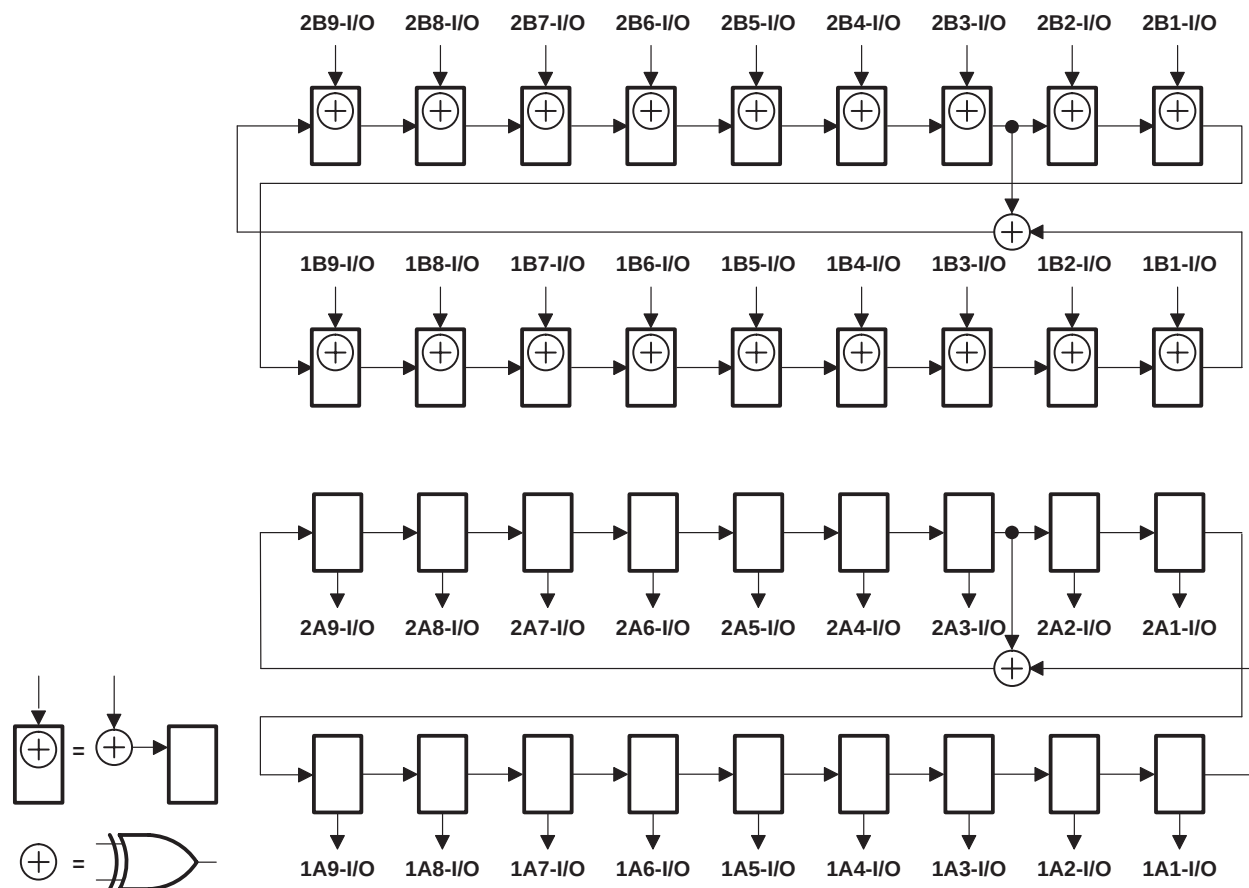
Figure 11. 18-Bit PSA/PRPG Configuration (10EAB = 20EAB = 0, \overline{1OEBA} = \overline{2OEBA} = 0 )
