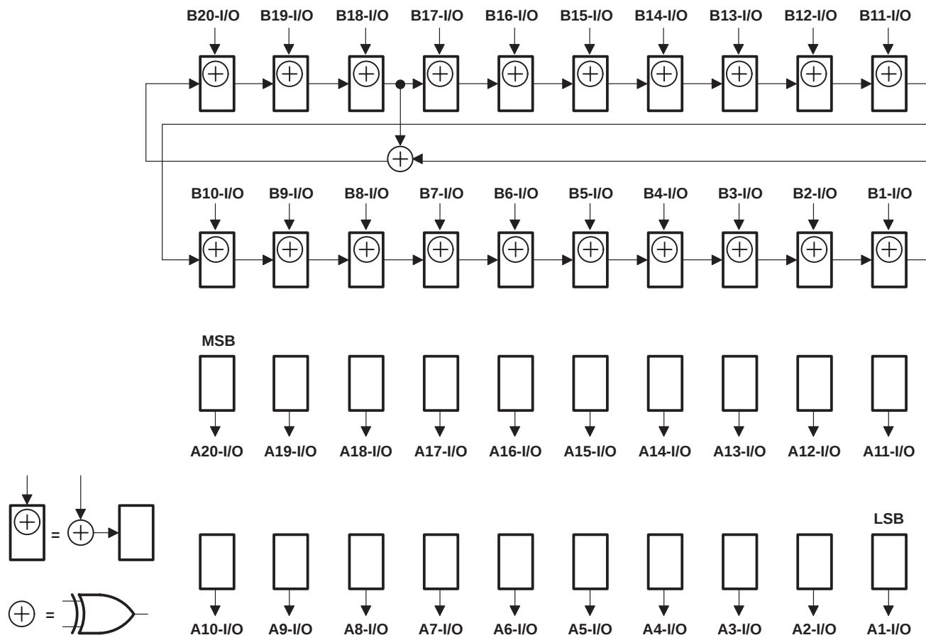
Figure 12. 20-Bit PSA/COUNT Configuration ( \overline{\text{OEAB}} = 1 , \overline{\text{OEBA}} = 0 )
