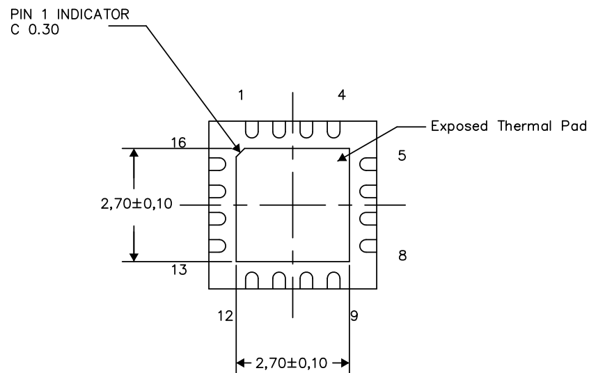
Bottom View
