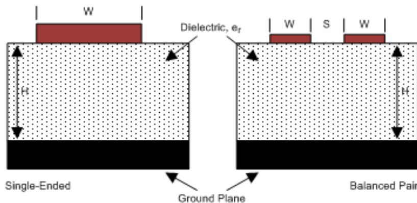
Figure 11-1. Microstrip Topology
