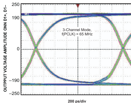
Figure 6-11. Data Eye Pattern, 3-channel Mode
