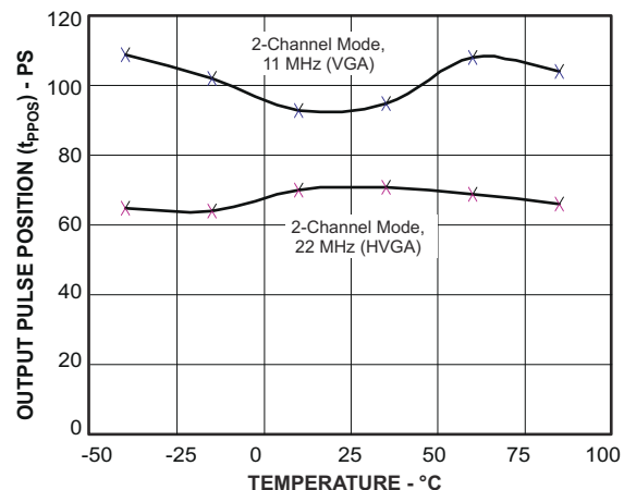
Figure 6-9. Output Pulse Position vs Temperature
