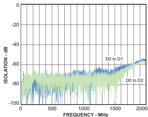
Figure 6-21. Crosstalk
