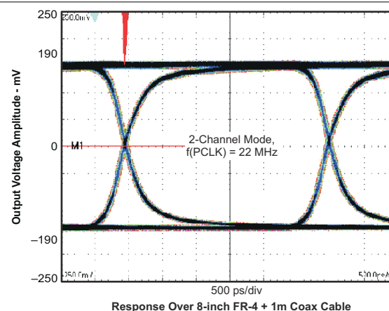
Figure 6-13. VGA 2-channel Output Waveform
