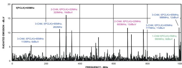
Figure 6-22. GTEM SAE J1752/3 EMI Test
