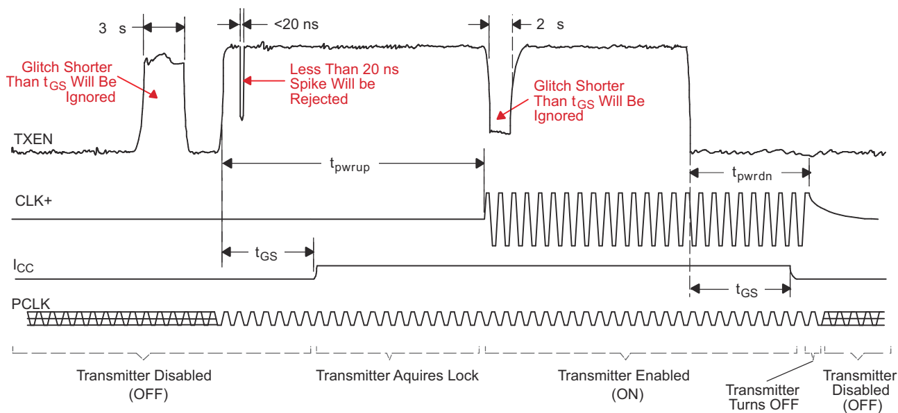
Figure 7-8. Transmitter Enable Glitch Suppression Time
