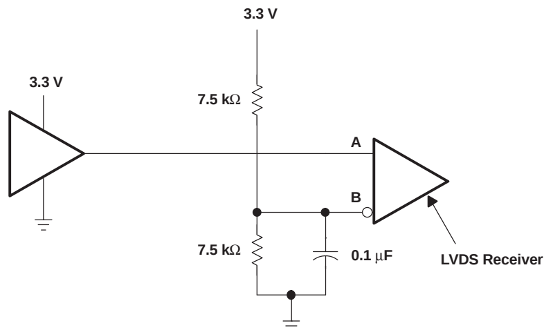
Figure 33. 3.3-V CMOS
