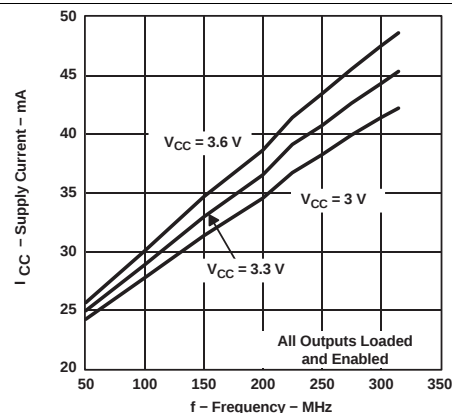
Figure 2. SN65LVDS105 Supply Current vs Frequency
