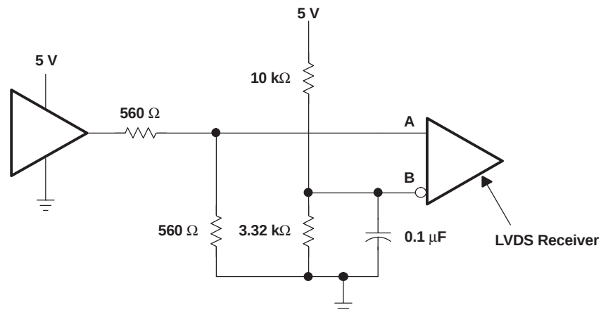
Figure 34. 5-V CMOS
