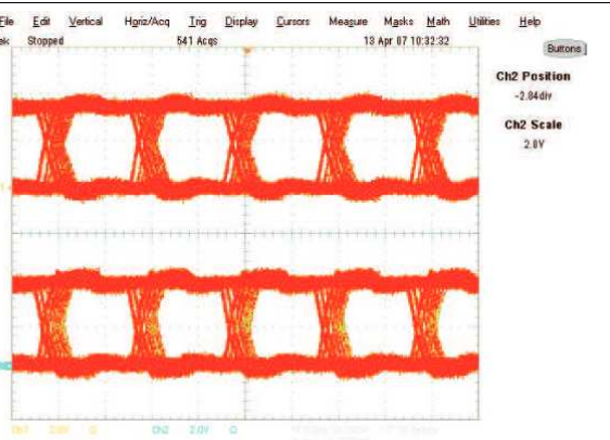
Figure 32. Typical Eye Pattern SN65LVDS050: Tx Buffers
