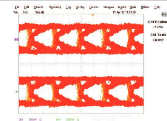
Figure 33. Typical Eye Pattern SN65LVDS051: All Buffers
