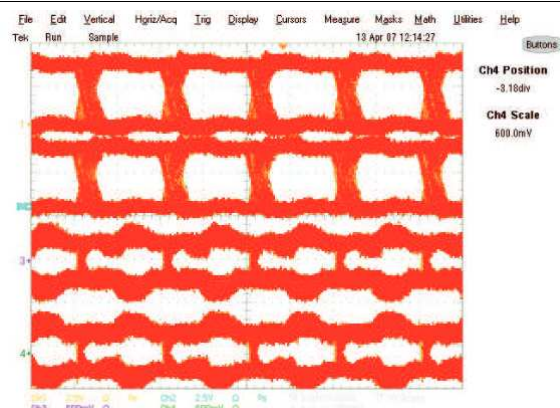
Figure 31. Typical Eye Pattern SN65LVDS050: Rx Buffers
