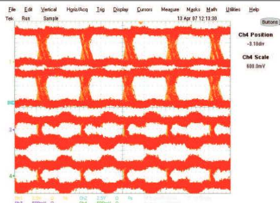
Figure 30. Typical Eye Pattern SN65LVDS050: All Buffers
