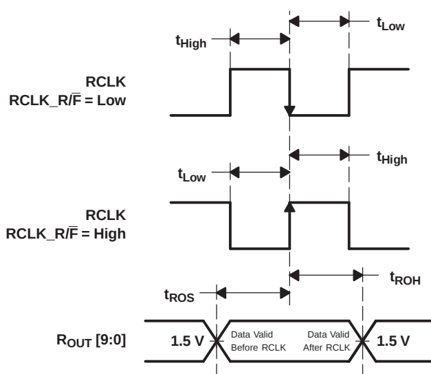
Figure 15. Deserializer Data Valid Out Times
