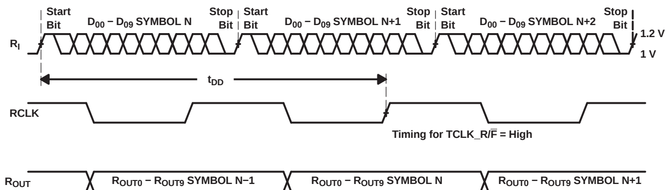
Figure 14. Deserializer Delay
