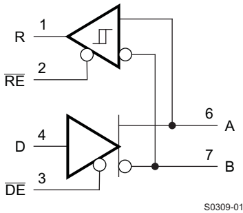
Figure 12. SN65HVD1708E Transceiver for J1708 Applications
