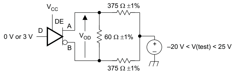
Figure 2. Measurement of Driver Differential Output Voltage With Common-Mode Load
