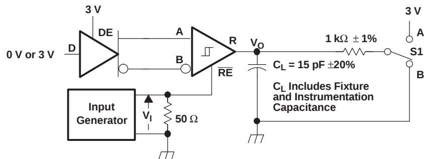
Figure 17. Receiver Switching Test Circuit and Voltage Waveforms
