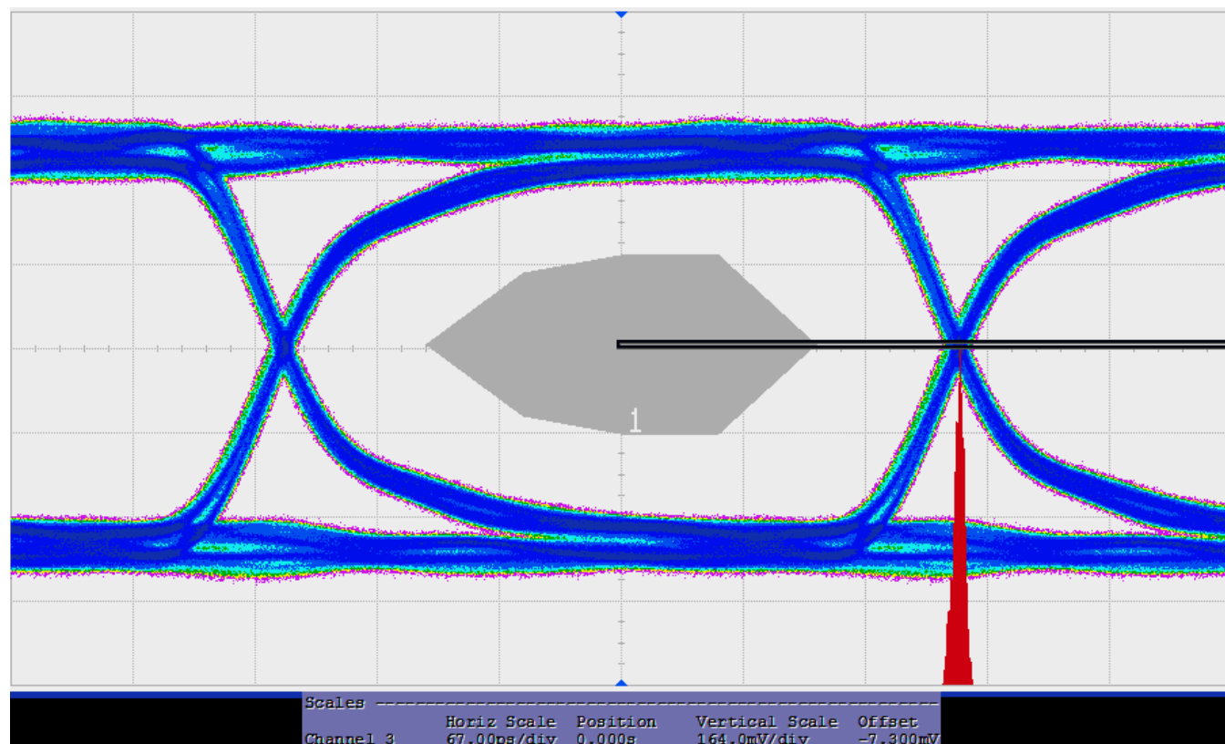
Figure 21. HBR Eye Diagram
