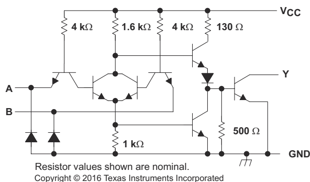
Figure 8-11. SNx5453B Schematic (Each Driver)
