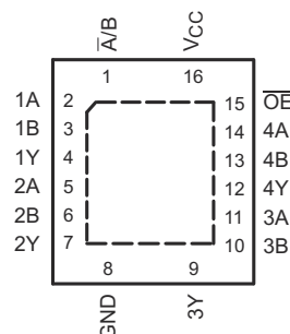
Figure 4-2. BQB or RGY Package; 16-Pin WQFN or VQFN with Exposed Thermal Pad (Top View)
