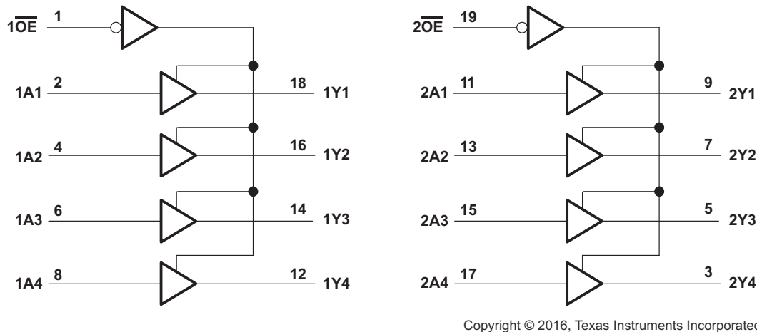
Figure 7-1. Logic Diagram (Positive Logic)
