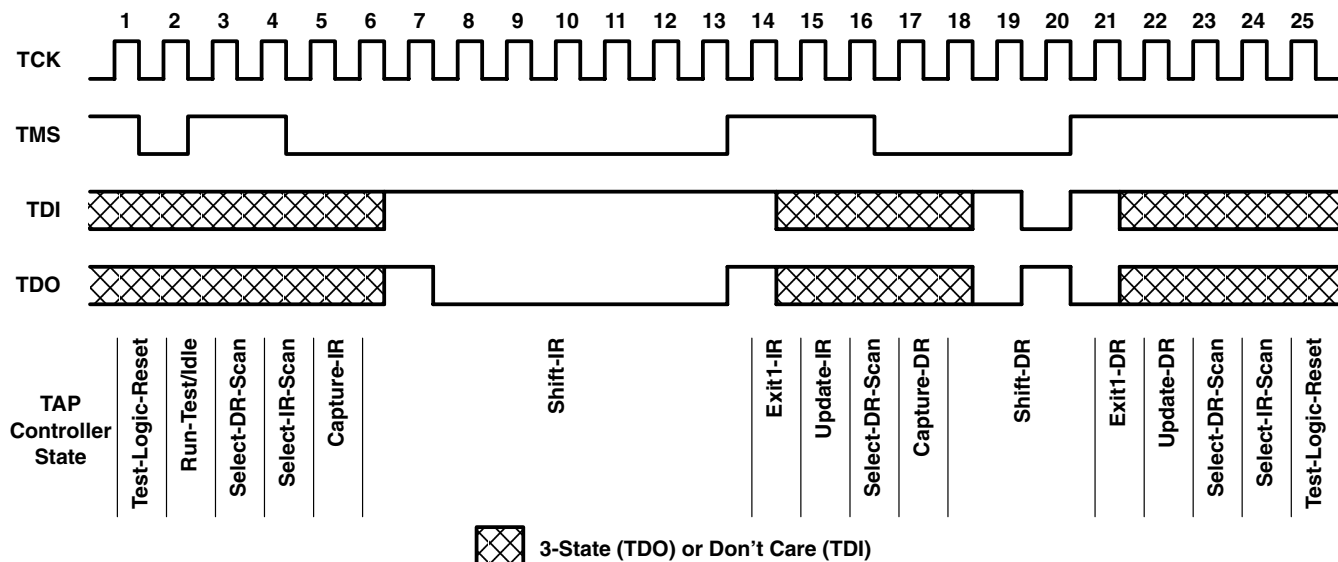
Figure 8. Timing Example
