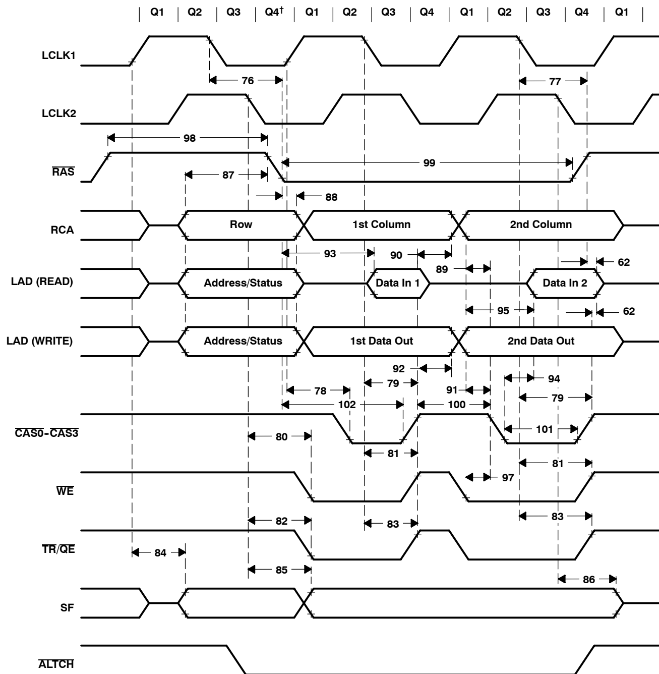
Figure 49. Local-Bus Timing: \overline{\text{RAS}} , \overline{\text{CAS0-CAS3}} , \overline{\text{WE}} , \overline{\text{TR/QE}} , and SF
