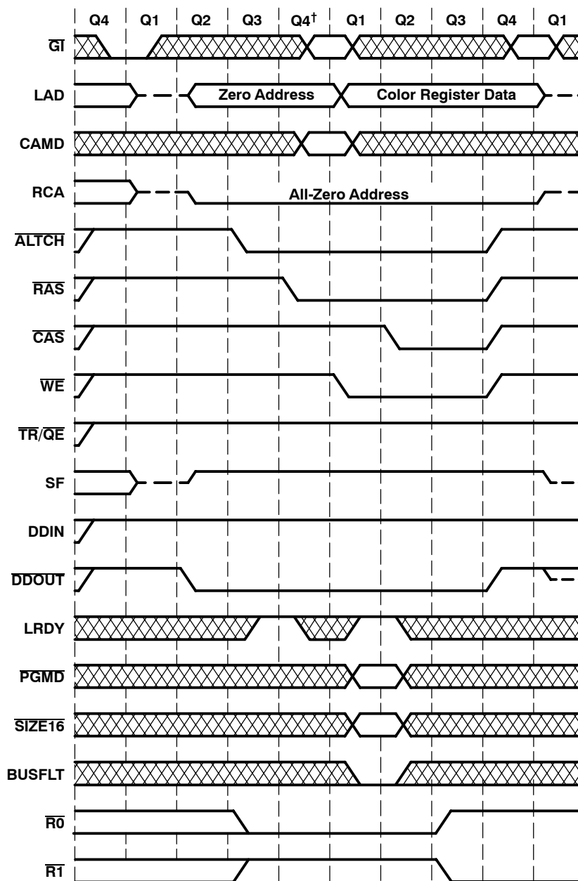
Figure 17. Load-Color-Latch-Cycle Timing
