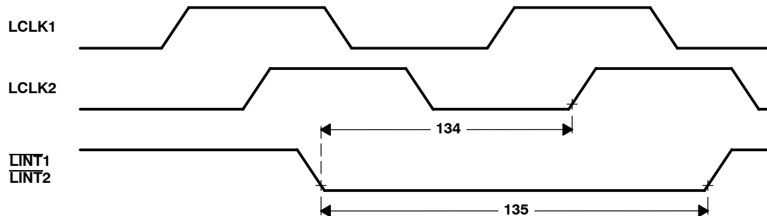
Figure 56. Interrupt Timing: \overline{LINT1} and \overline{LINT2}
