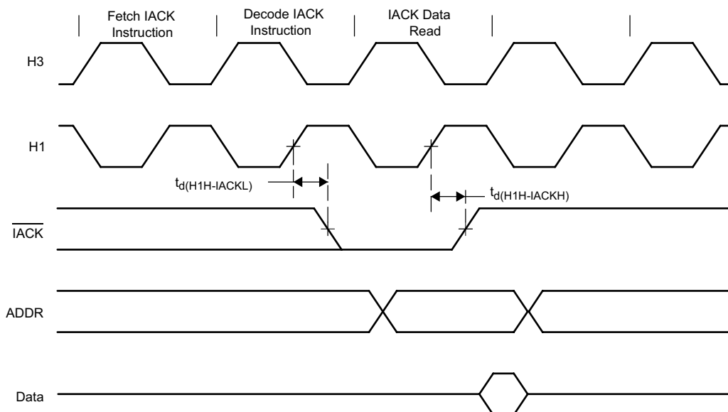
Figure 16. Interrupt Acknowledge ( \overline{\text{IACK}} ) Timing
