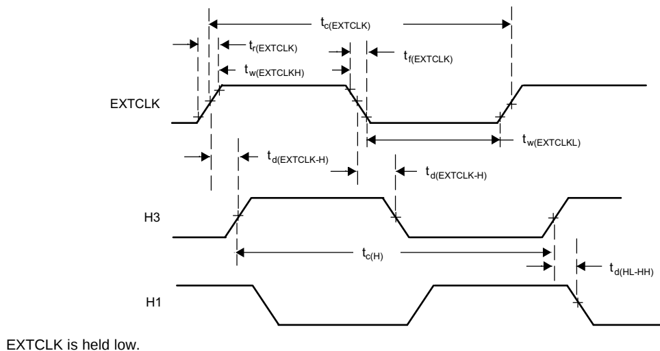
Figure 4. Divide-by-One Mode
