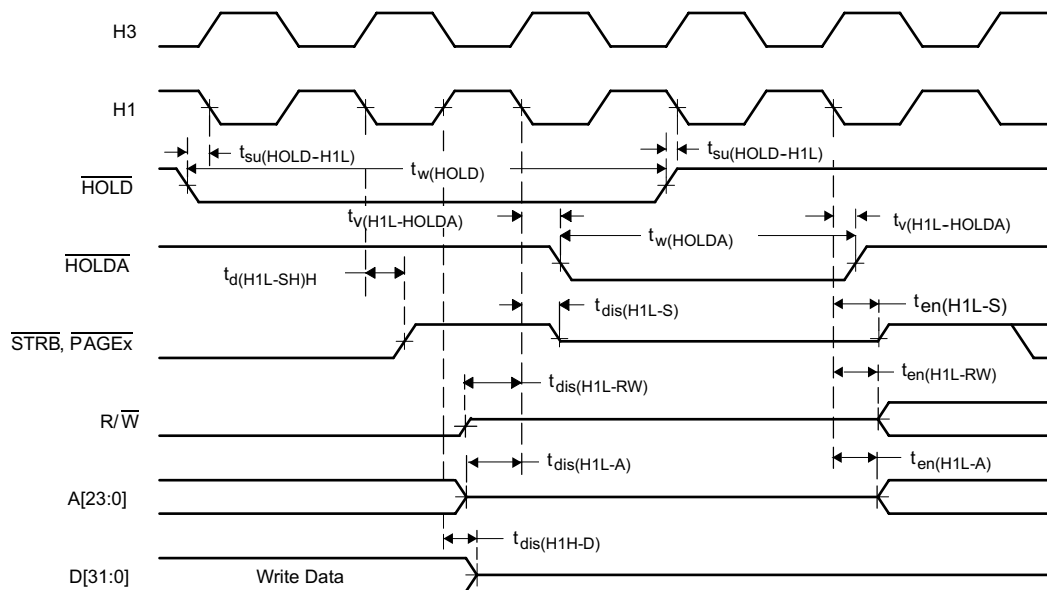
Figure 17. Timing for \overline{HOLD}/\overline{HOLDA} (After Write)
