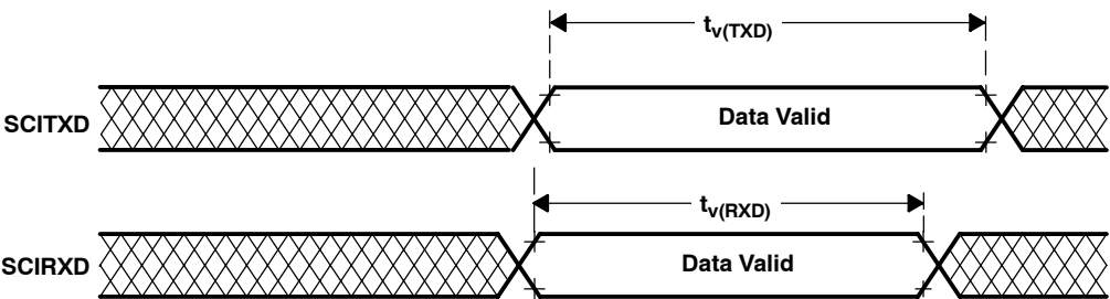
Figure 43. SCI Timings
