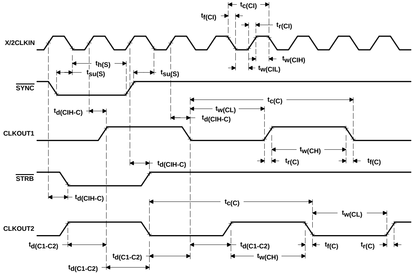
Figure 5. Clock Timing
