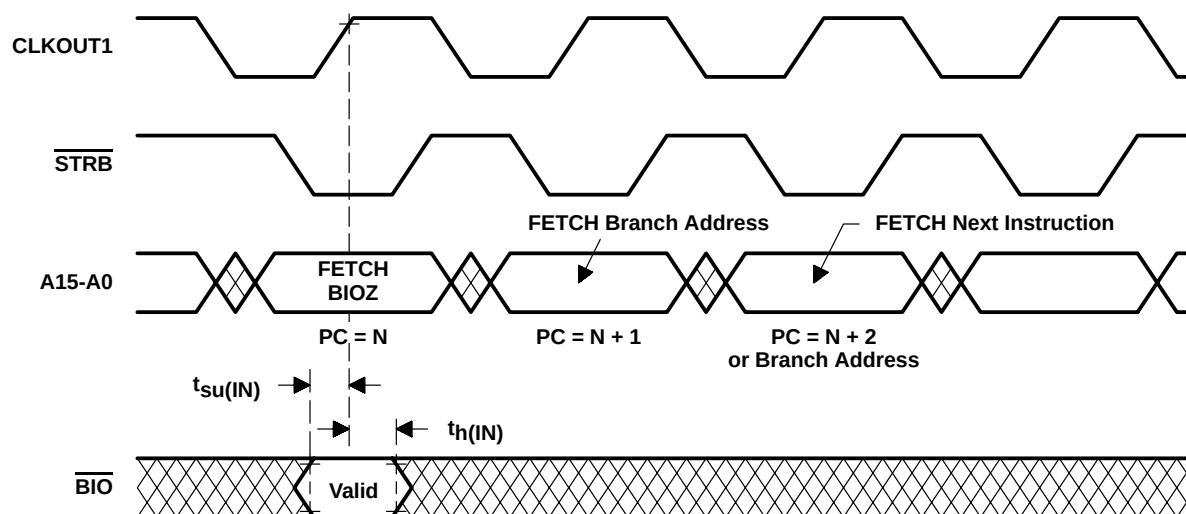
Figure 11. BIO Timing
