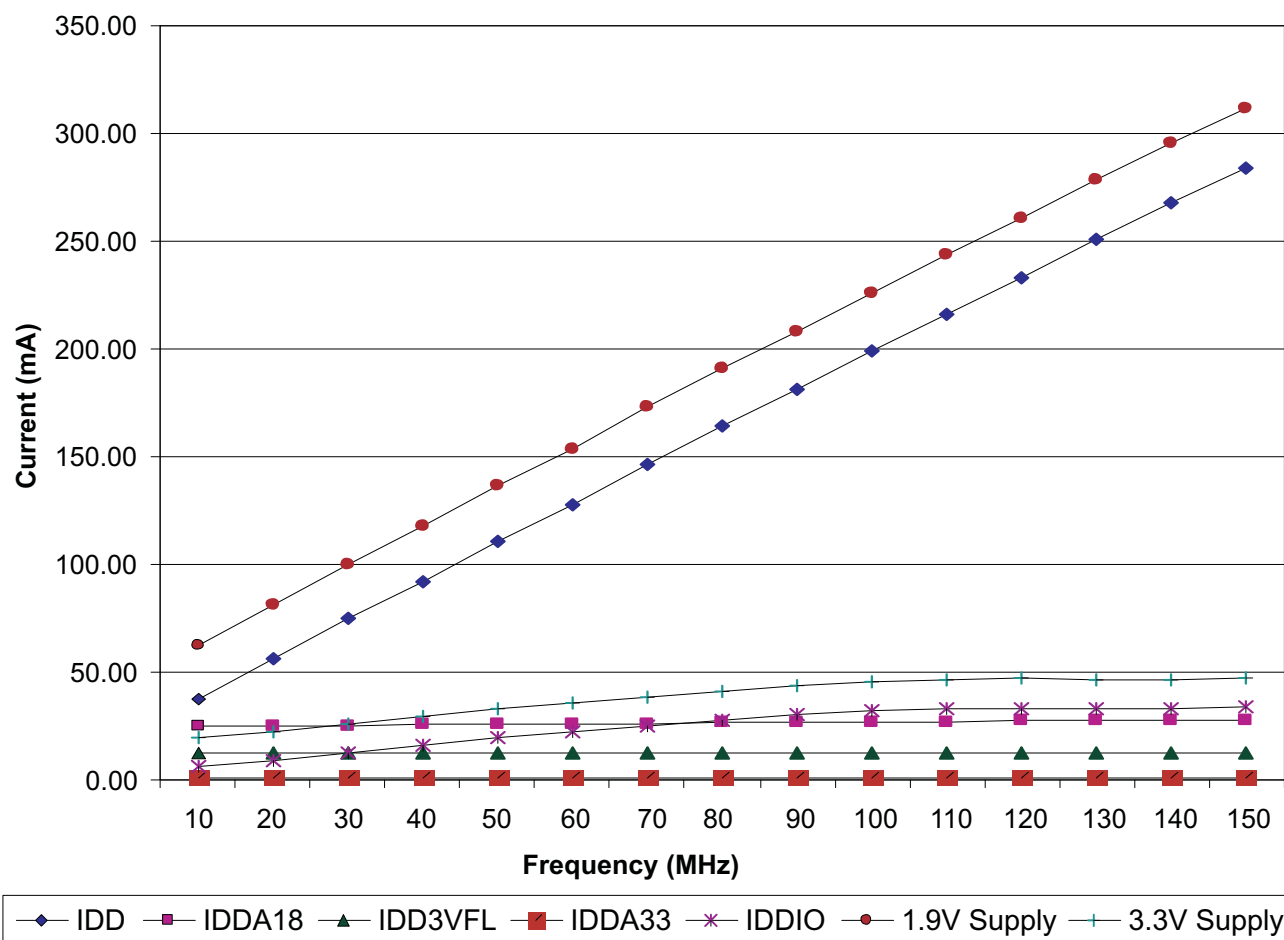
Figure 6-3. Typical Operational Current Versus Frequency for T_A = 25^\circ\text{C}
