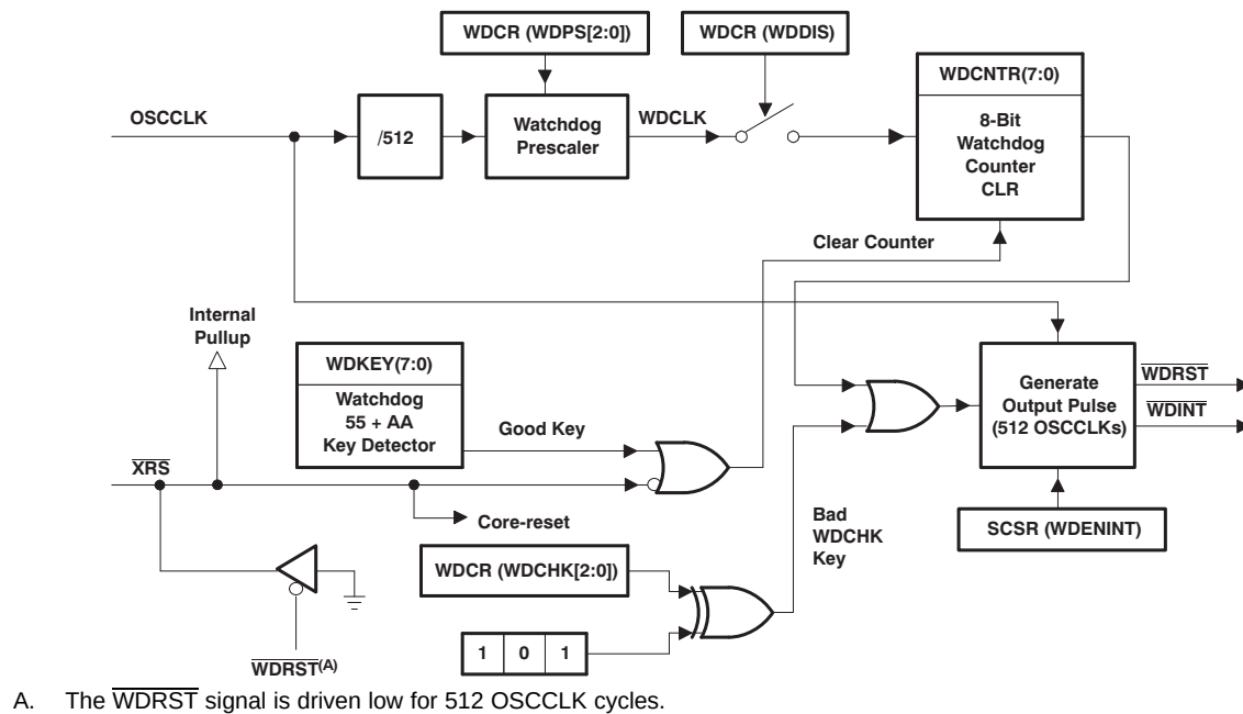
Figure 3-11. Watchdog Module
