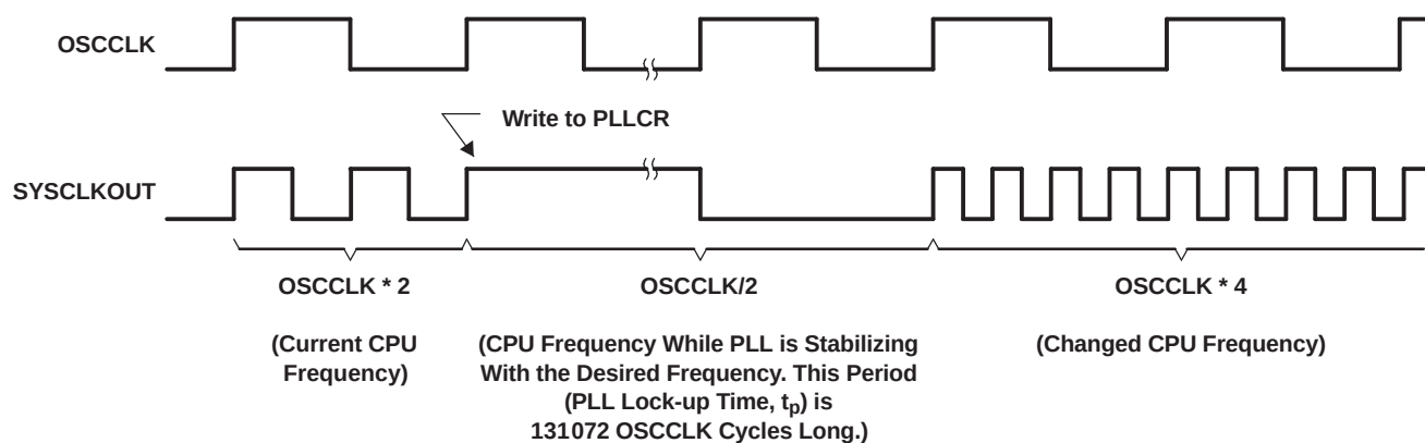
Figure 6-11. Example of Effect of Writing Into PLLCR Register
