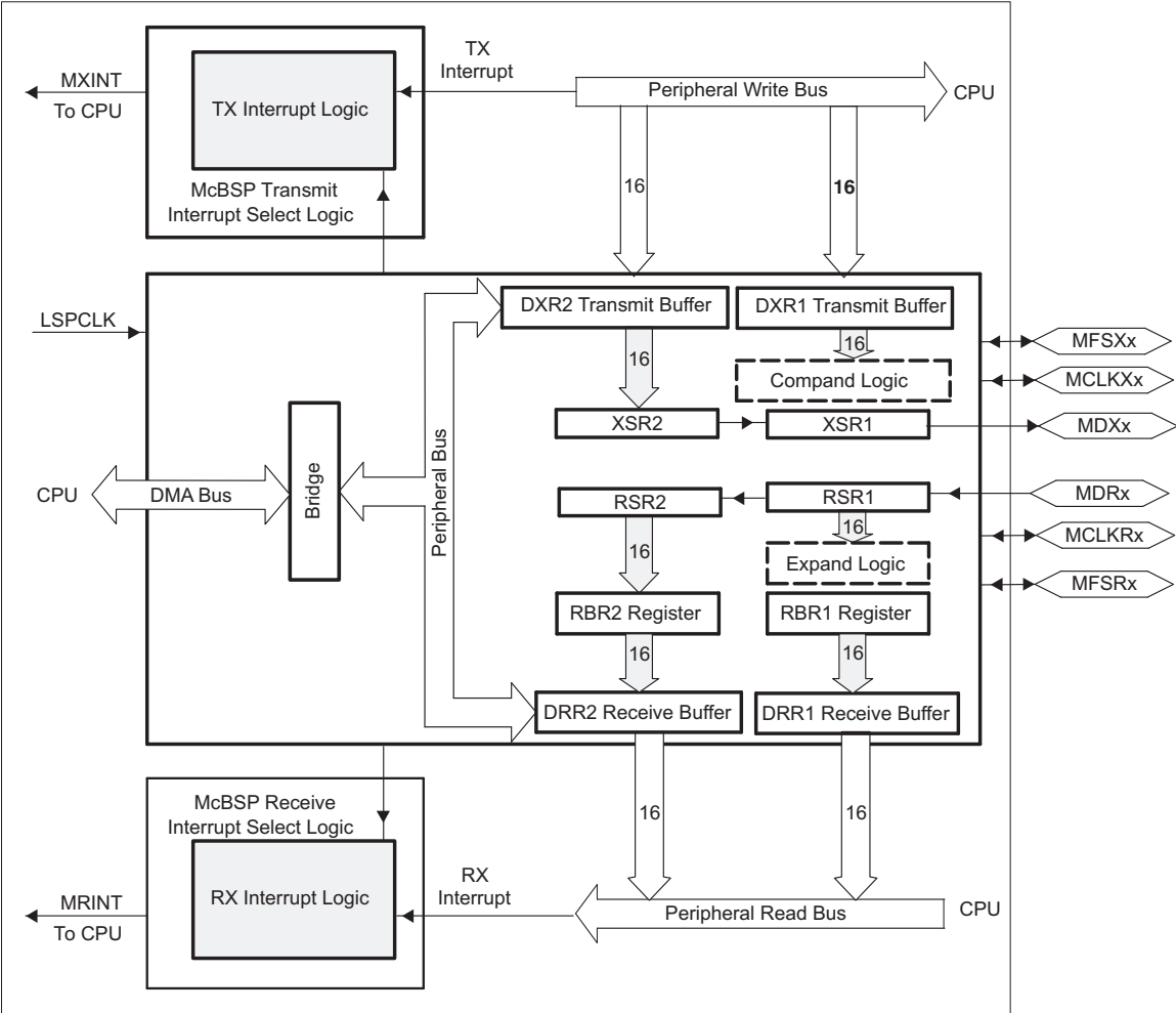
Figure 4-11. McBSP Module
