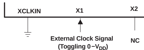
Figure 3-9. Using a 1.9-V External Oscillator
