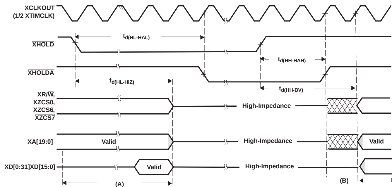
Figure 6-33. \overline{\text{XHOLD}}/\overline{\text{XHOLDA}} Timing Requirements ( \text{XCLKOUT} = 1/2 \text{ XTIMCLK} )
