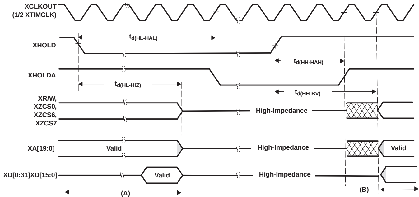
Figure 6-31. \overline{\text{XHOLD}}/\overline{\text{XHOLDA}} Timing Requirements ( \text{XCLKOUT} = 1/2 \text{XTIMCLK} )
