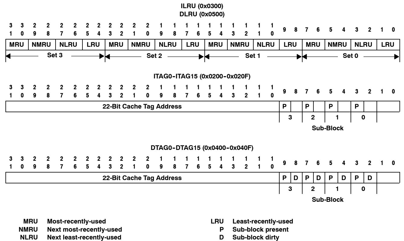
Figure 17. Cache Registers
