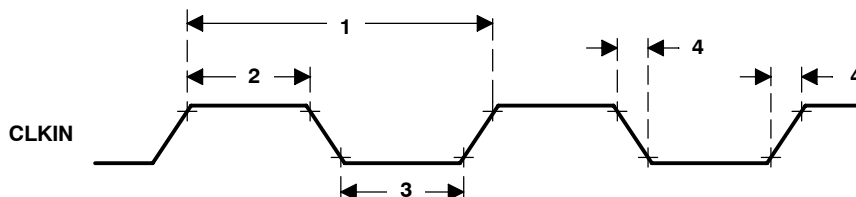
Figure 108. CLKIN Timing
