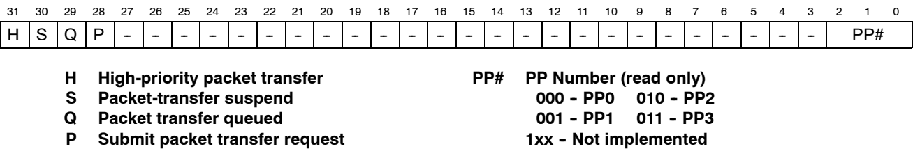
Figure 32. comm Register
