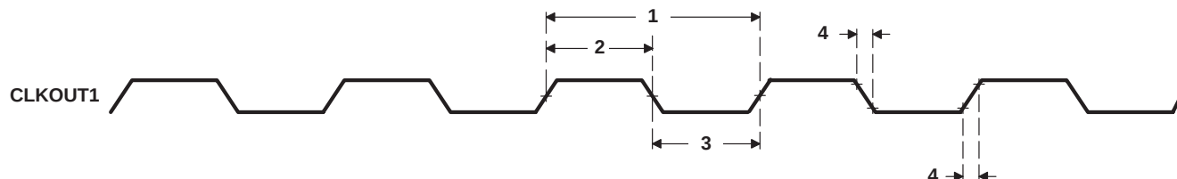
Figure 9. CLKOUT1 Timings
