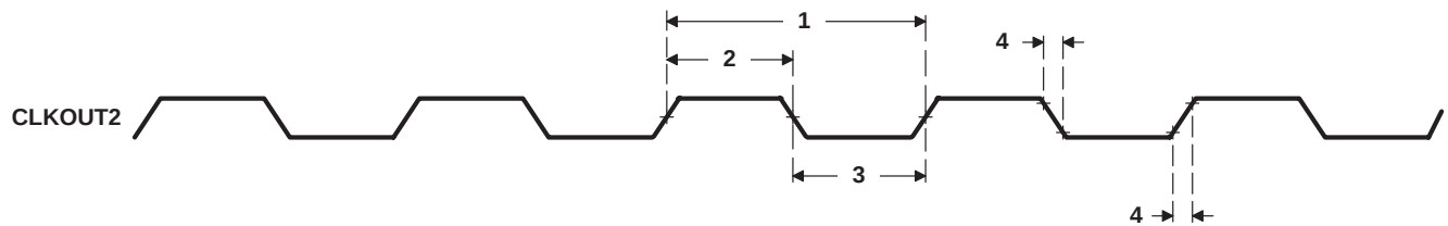
Figure 10. CLKOUT2 Timings
