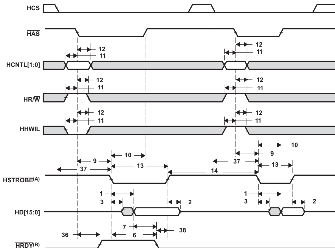
Figure 4-44. HPI16 Read Timing ( \overline{HAS} Used)
