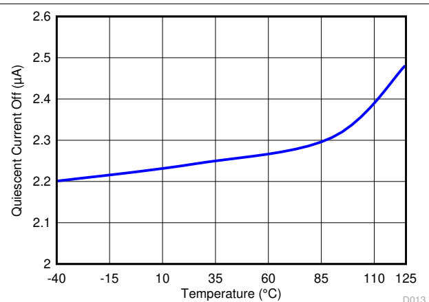
Figure 9-3. Quiescent Current Shutdown Mode
