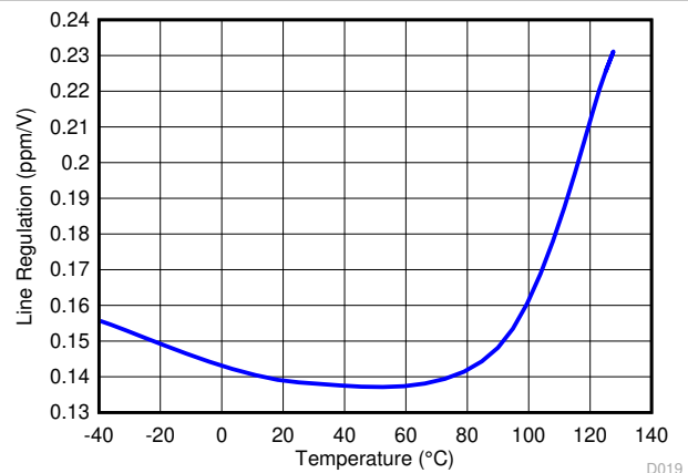
Figure 6-6. Line Regulation
