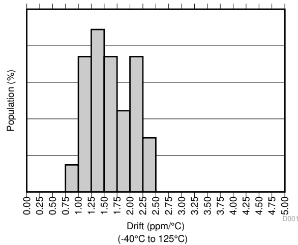
Figure 6-1. Temperature Drift
