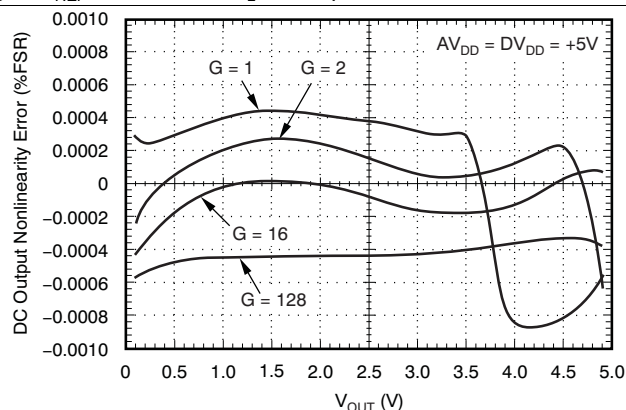
Figure 10. PGA112 and PGA116 Nonlinearity
