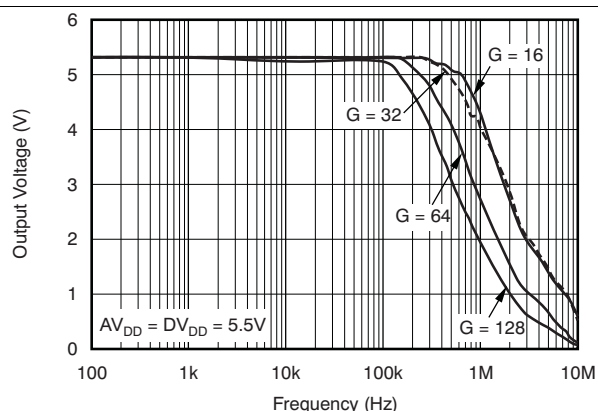
Figure 34. PGA112, PGA116 Output Voltage Swing vs Frequency
