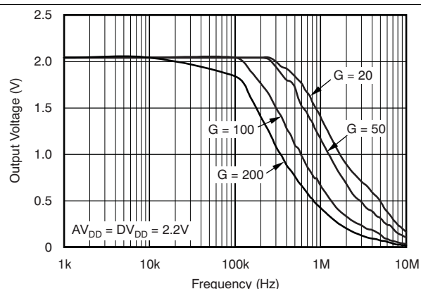
Figure 36. PGA112, PGA116 Output Voltage Swing vs Frequency
