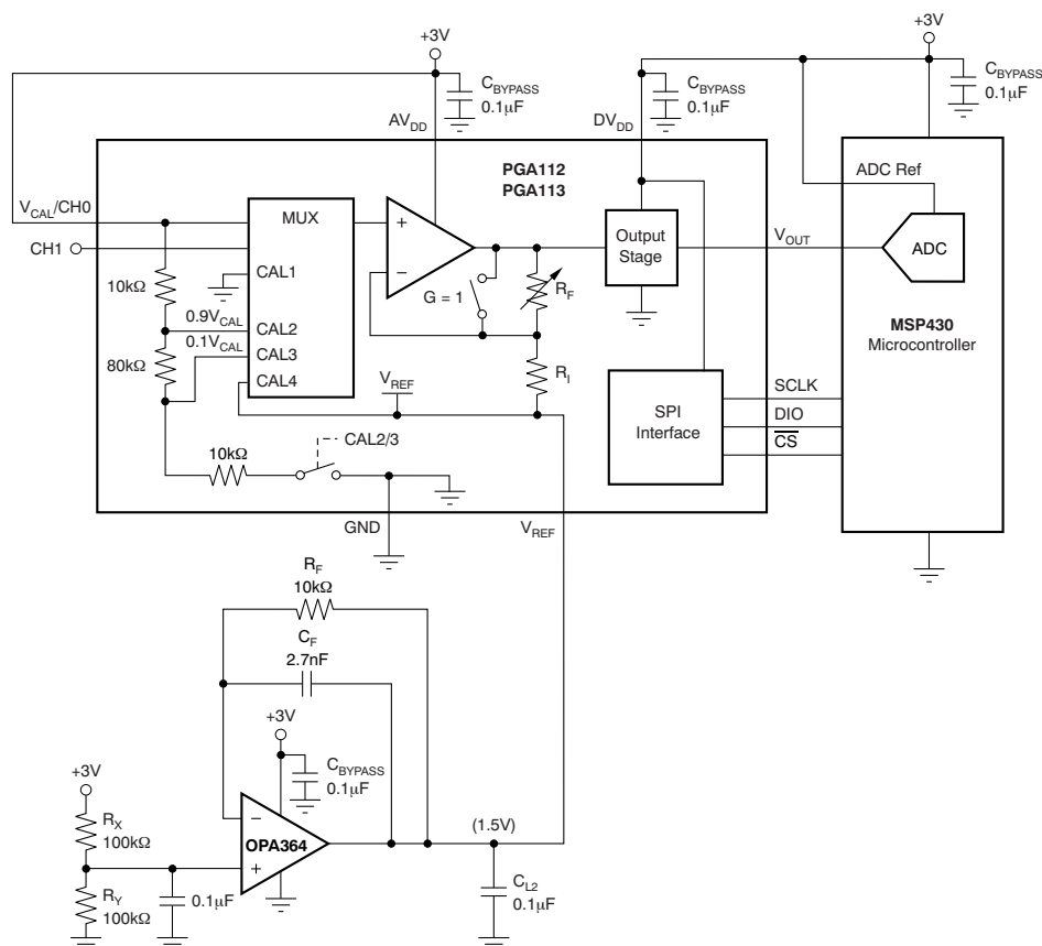
FUNCTION MUX SELECT GAIN SELECT MUX INPUT OP AMP (+In) OP AMP (V OUT ) DESCRIPTION Minimum Signal CAL1 1 GND GND 50 mV Minimum signal level that the MUX, op amp, and ADC can read. Op amp V OUT is limited by negative saturation. Gain Calibration CAL2 1 0.9 \times (V_{\text{CAL}}/\text{CH0}) 2.25 V 2.25 V 90% ADC Ref for system full-scale or gain calibration of the ADC. Maximum Signal CAL2 2 0.9 \times (V_{\text{CAL}}/\text{CH0}) 2.25 V 2.95 V Maximum signal level that the MUX, op amp, and ADC can read. Op amp V OUT is limited by positive saturation. System is limited by ADC max input of 2.5 V (ADC Ref = 2.5 V). Offset Calibration CAL3 1 0.1 \times (V_{\text{CAL}}/\text{CH0}) 0.25 V 0.25 V 10% ADC Ref for system offset calibration of the ADC. Minimum Signal CAL4 1 V REF GND 50 mV Minimum signal level that the MUX, op amp, and ADC can read. Op amp V OUT is limited by negative saturation.
