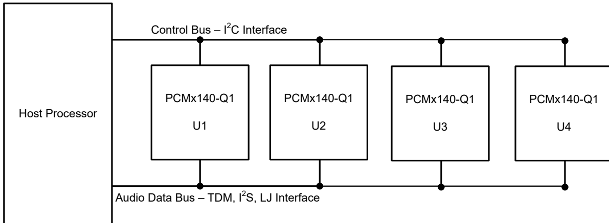
Figure 7-13. Multiple PCM5140-Q1 Devices With Shared Control and Audio Data Buses
