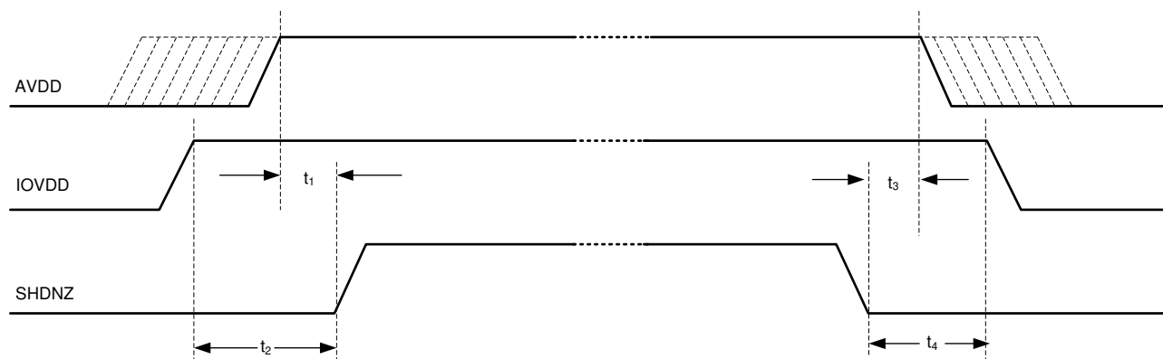
Figure 8-7. Power-Supply Sequencing Requirement Timing Diagram
