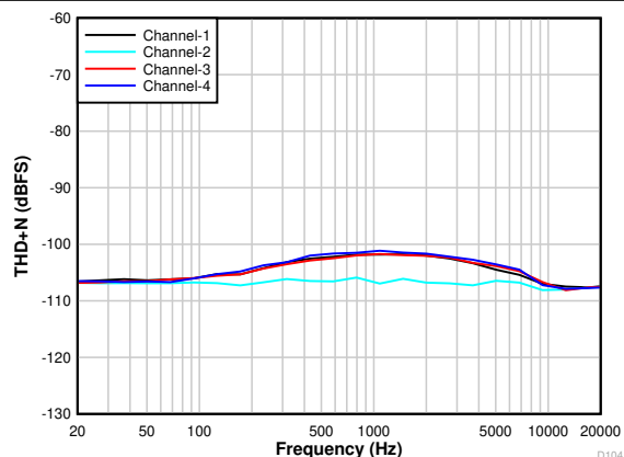
Figure 6-12. THD+N vs Input Frequency With a -1-dBr Input
