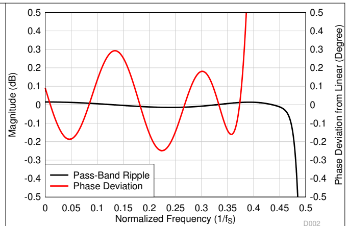
Figure 7-44. Low-Latency Decimation Filter Pass-Band Ripple and Phase Deviation
