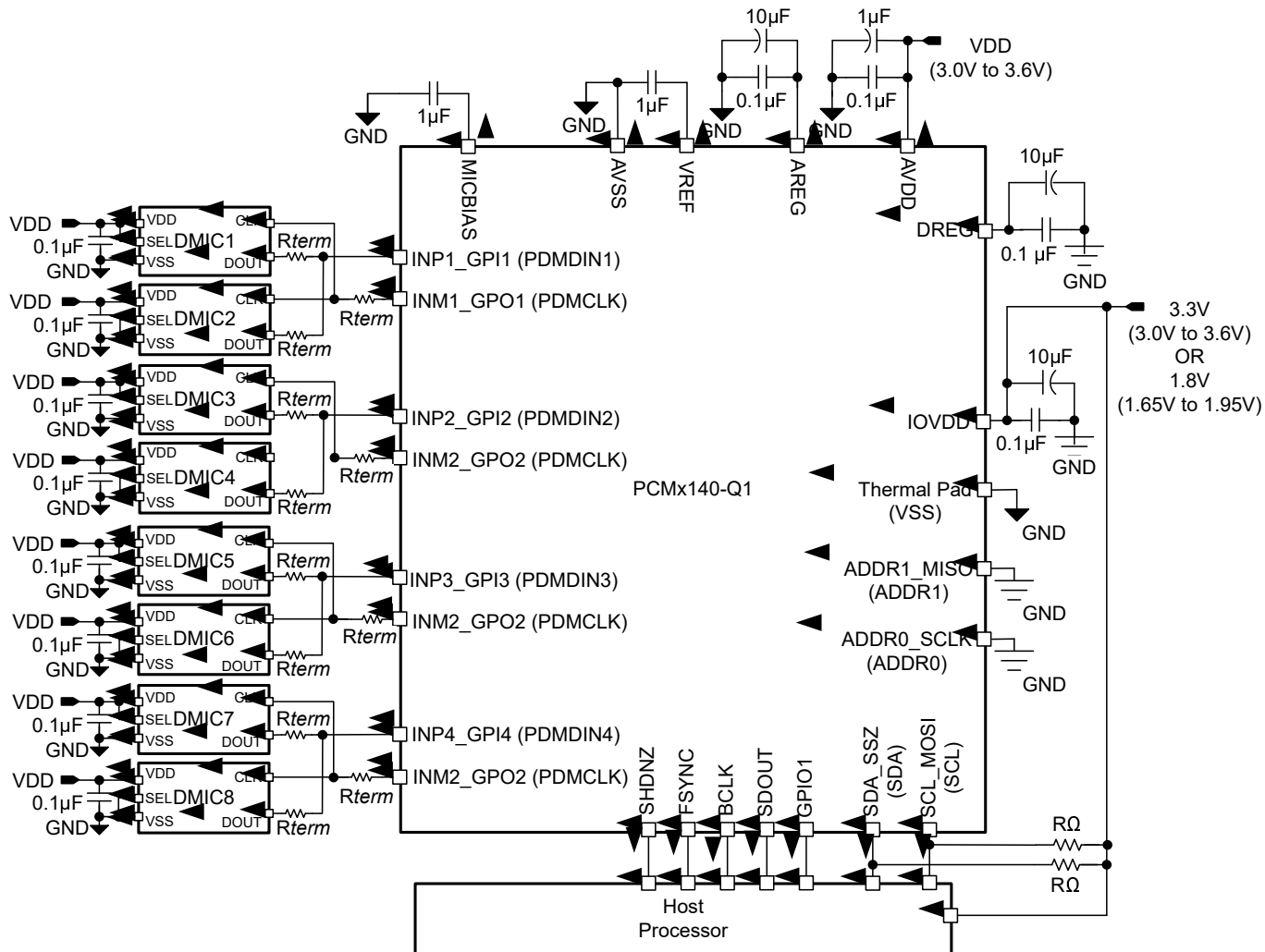
Figure 8-6. Eight-Channel Digital PDM Microphone Recording Diagram
