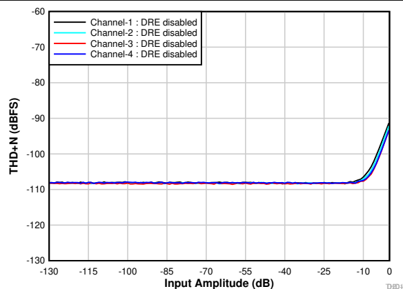
Figure 8-5. THD+N vs Input Amplitude With DRE Disabled
