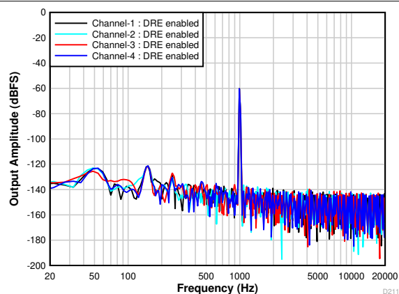
Figure 8-2. FFT With a -60-dBr Input With DRE Enabled
