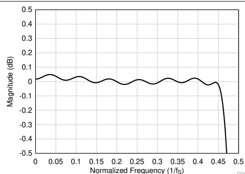
Figure 7-20. Linear Phase Decimation Filter Pass-Band Ripple
