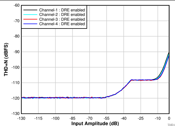
Figure 8-3. THD+N vs Input Amplitude With DRE Enabled
