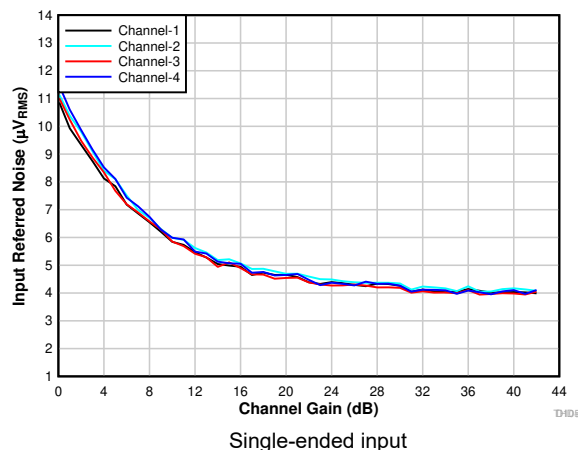
Figure 6-14. Input-Referred Noise vs Channel Gain
