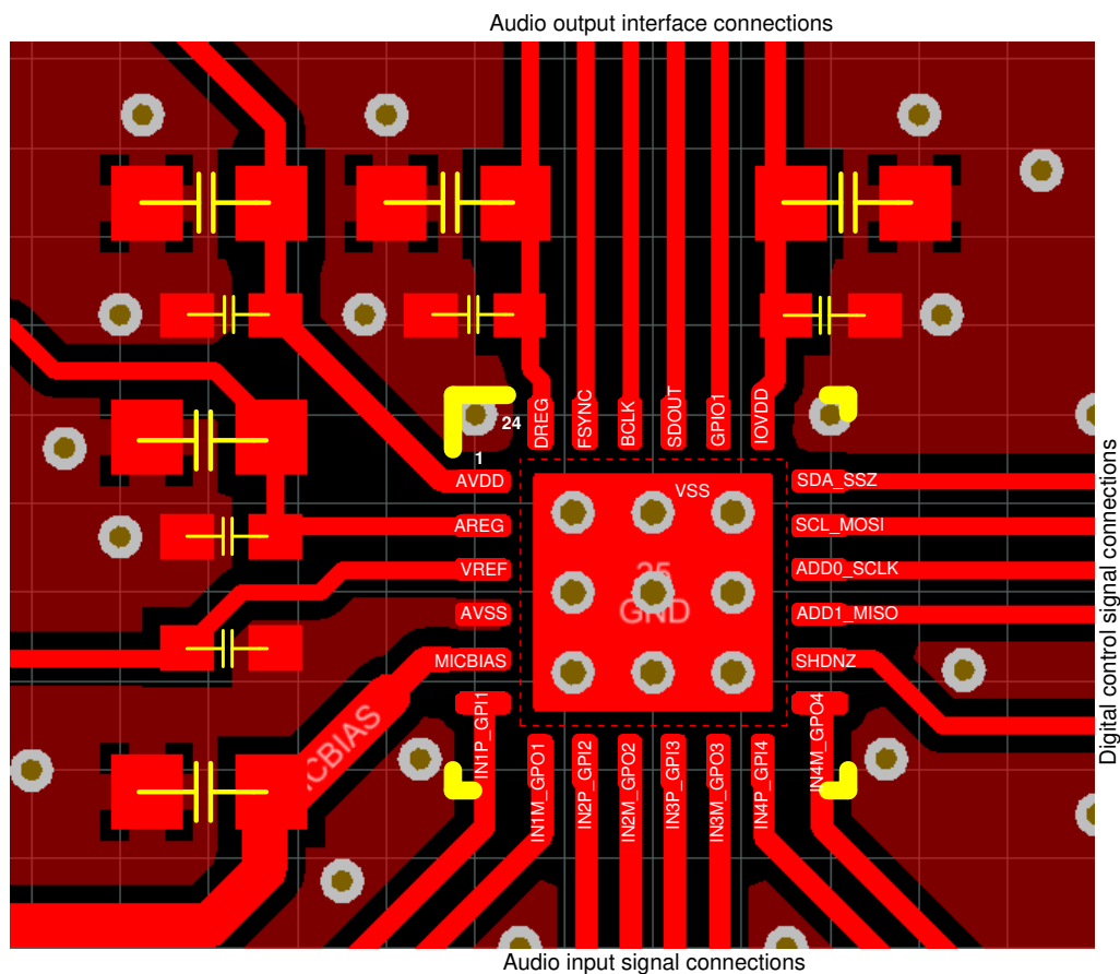
Figure 8-8. Layout Example
