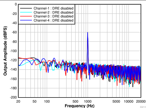
Figure 8-4. FFT With a -60-dBr Input With DRE Disabled
