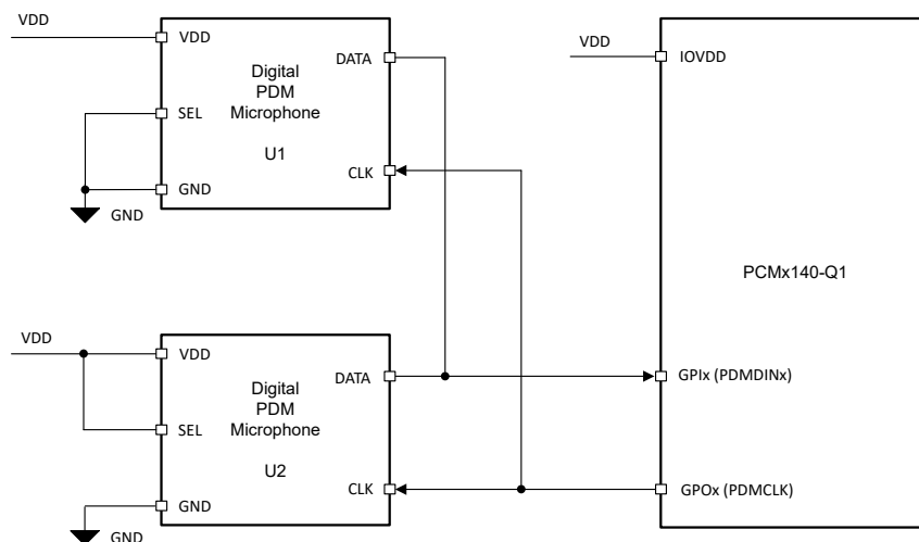
Figure 7-64. Digital PDM Microphones Connection Diagram to the PCM5140-Q1
