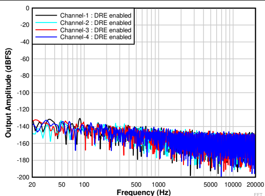
Figure 6-17. FFT With Idle Input With DRE Enabled
