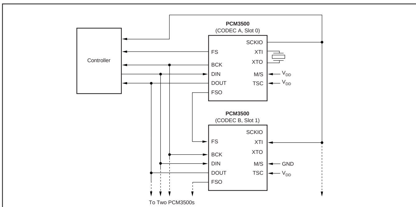
FIGURE 11. Time Slot Mode Connections.
