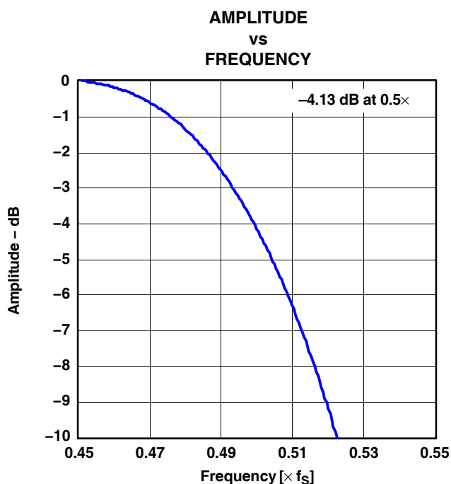
Figure 4. Transition-Band Characteristics
