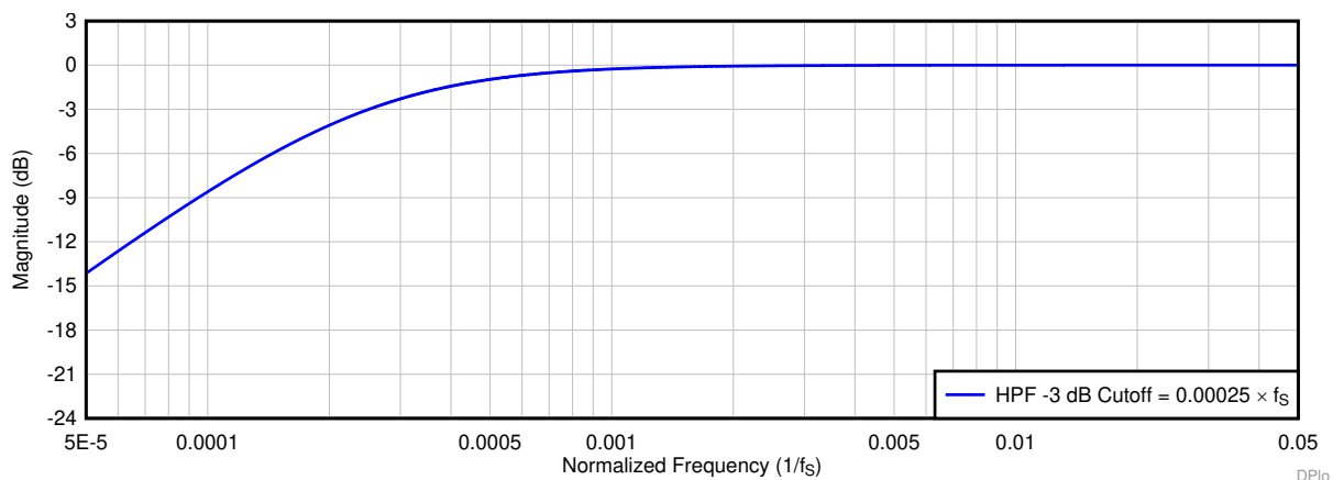
Figure 23. HPF Filter Frequency Response Plot
