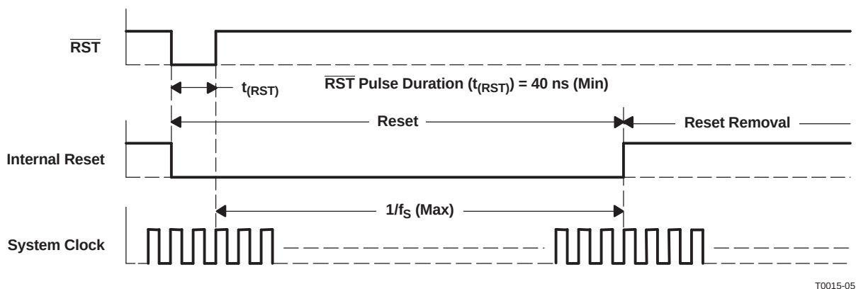
Figure 34. External Reset Timing
