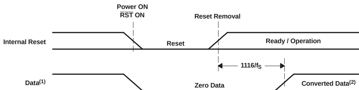
Figure 34. External Reset Timing
