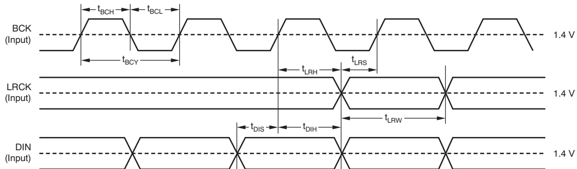
Figure 35. Audio Interface Timing Diagram for Left-Justified, Right-Justified, I²S, and DSP Data Formats
