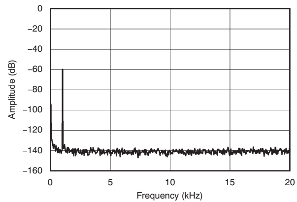
Figure 17. Output Spectrum
