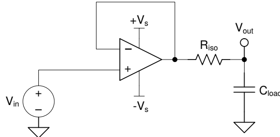
Figure 6-7. Extending Capacitive Load Drive With the OPAx991-EP
