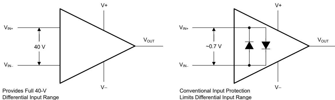
Figure 6-1. OPAx991-EP Input Protection Does Not Limit Differential Input Capability
