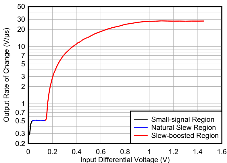
Figure 7-1. Output Rate of Change vs Input Differential Voltage for the OPAX991-EP
