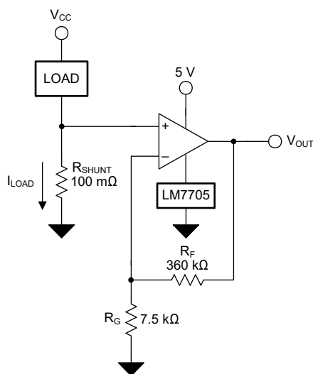
Figure 7-4. OPAx991-EP in a Low-Side, Current-Sensing Application
