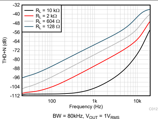
Figure 5-21. THD+N Ratio vs Frequency
