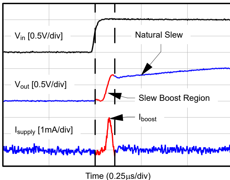
Figure 7-2. Large-Signal Step Response Characteristics of the OPAX991-EP
