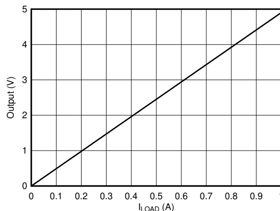
Figure 7-5. Low-Side, Current-Sense, Transfer Function
