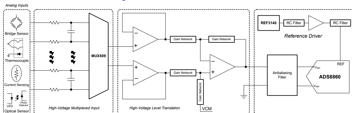
OPAx991-EP in a High-Voltage Signal Chain
