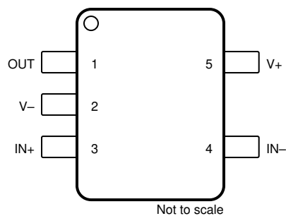
Figure 4-1. OPA991-EP DBV Package 5-Pin SOT-23 (Top View)
