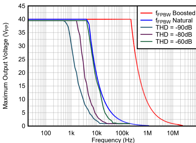
Figure 7-3. Maximum Output Voltage vs Frequency in Natural and Boosted Slew for the OPAX991-EP
