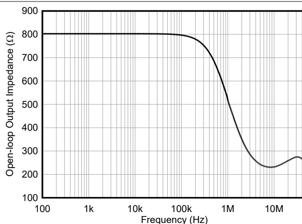
Figure 5-26. Open-loop Output Impedance vs Frequency
